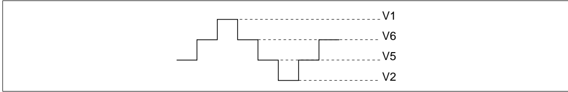
Figure 1 LCD Drive Levels
