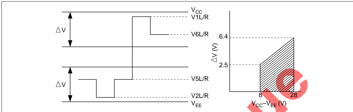
Figure 21 Relationship between Driver Output Waveform
