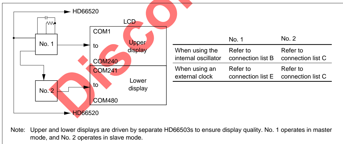
Figure 10 When Using Two HD66503s
