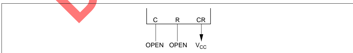
Figure 5 Oscillator Connection in Slave Mode
