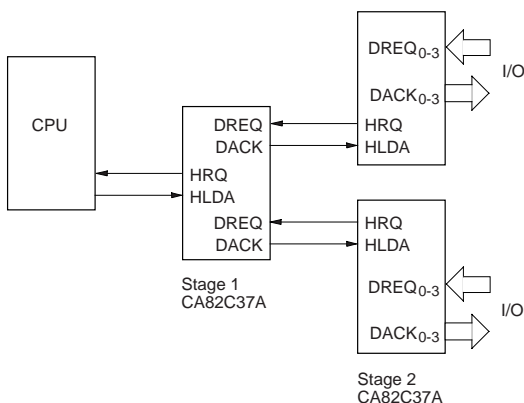
Figure 2-15: Cascaded CA82C37As
