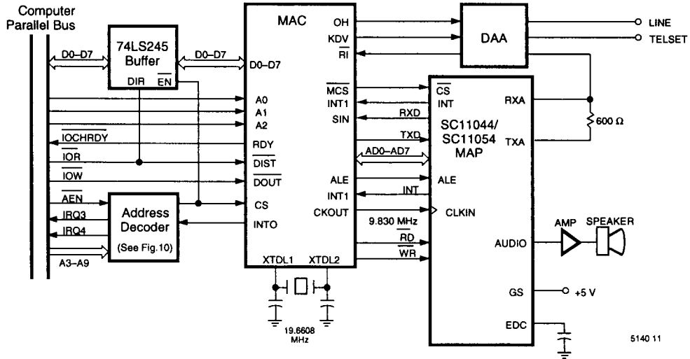
Figure 8. Internal Sendfax & Data Modem for PC Bus Applications with Internal ROM
