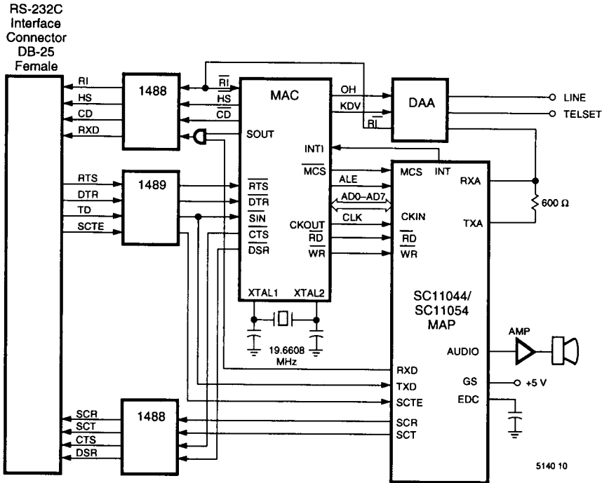
Figure 7. V.22bis Standalone Sendfax & Data Modem with Internal ROM
