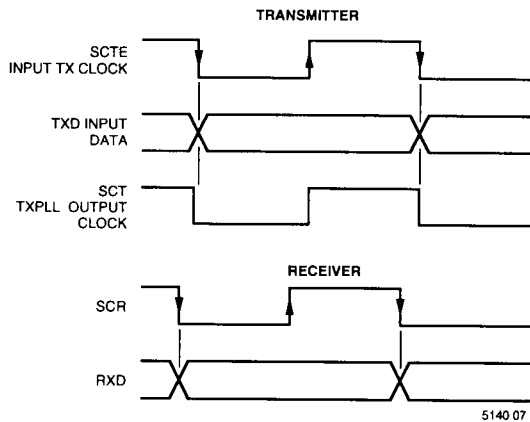
Figure 5. SC11044/SC11054 Synchronous Mode Timing Diagrams
