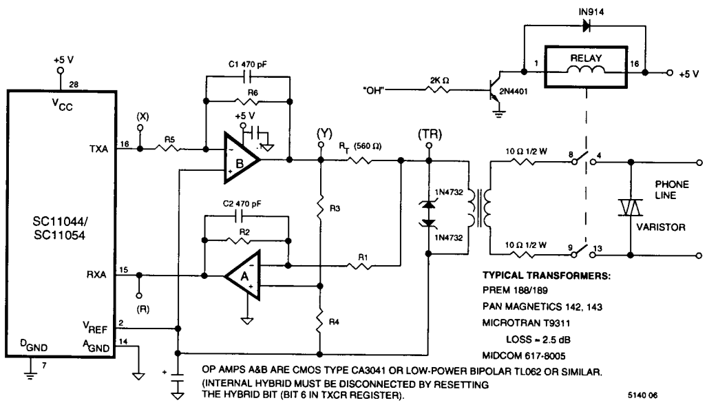
Figure 4. Using an External Hybrid with the SC11044/SC11054
