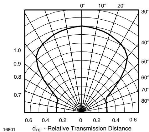
Fig. 12 - Directivity
