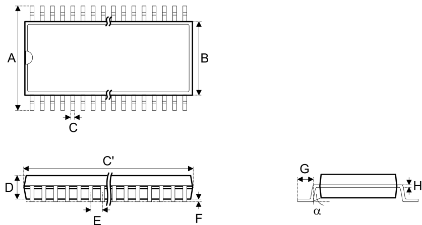
48 pin SSOP Outline dimensions
