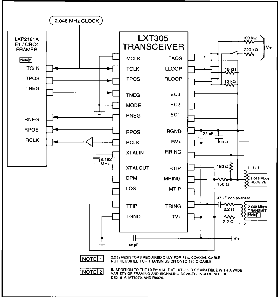
Figure 5: Typical LXT305 75 Ω E1 Application (Hardware Mode)
