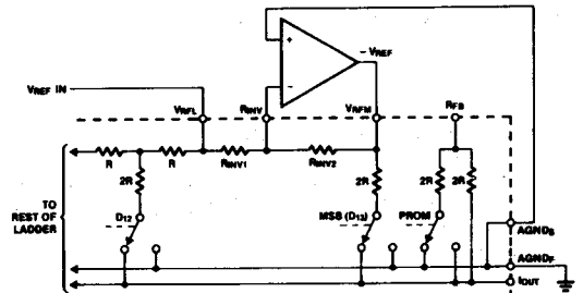
Figure 4. Bipolar Operation, with inverted V REF to MSB
