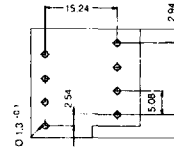
Pitch 5.08 mm
