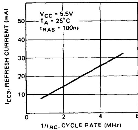
Fig. 10 - REFRESH CURRENT vs CYCLE RATE
