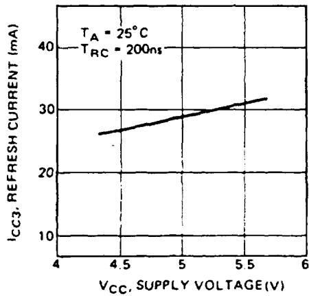
Fig. 11 - REFRESH CURRENT vs SUPPLY VOLTAGE
