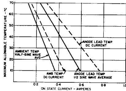
FIGURE 5. ON-STATE CURRENT VS. MAXIMUM ALLOWABLE TEMPERATURE
