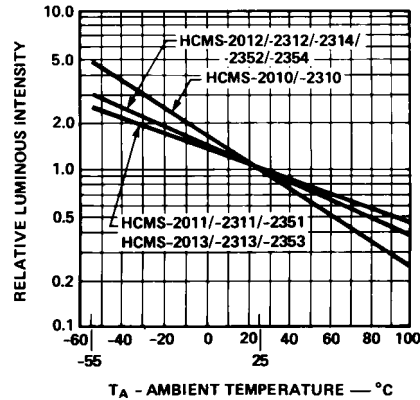
Figure 2. Relative Luminous Intensity vs Ambient Temperature.
