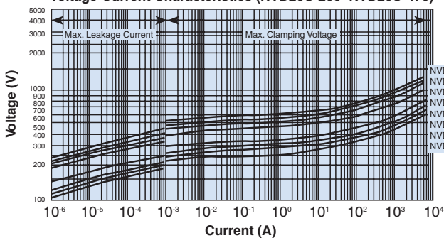
Voltage-Current Characteristics (NVD20U-200~NVD20U-470)
