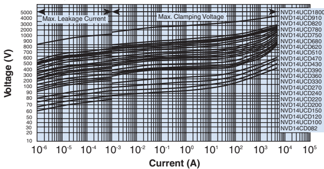
Voltage-Current Characteristics (NVD14U-082~NVD14U-1800)
