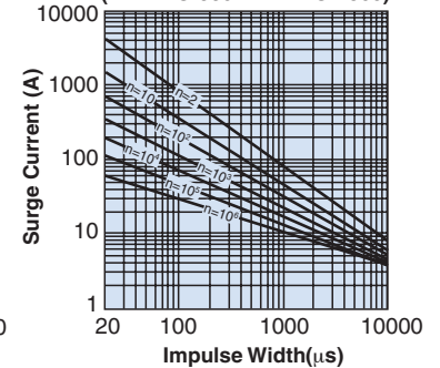
Image Derating (NVD14U-330~NVD14U-1800)
