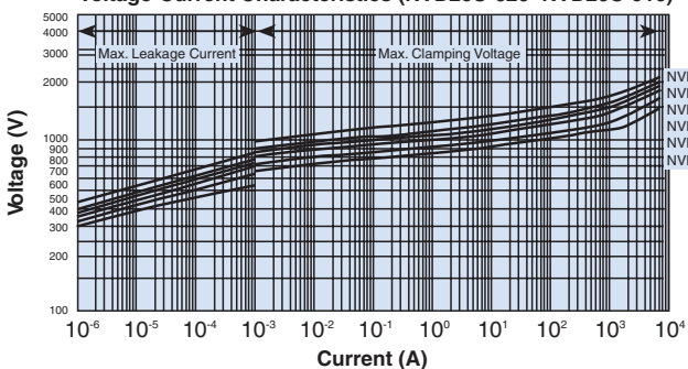
Voltage-Current Characteristics (NVD20U-620~NVD20U-910)
