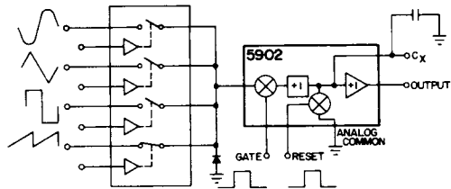
FIGURE 4: MULTIPLEX INPUT SIGNAL
