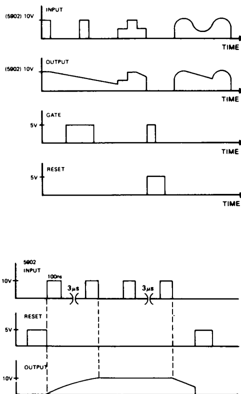
FIGURE 2: BASIC SIGNAL TIME RELATIONSHIPS
