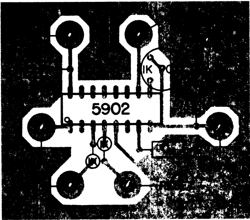
TYPICAL COMPONENT BOARD LAYOUT
