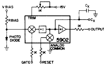
FIGURE 3: PEAK LIGHT LEVEL SENSING
