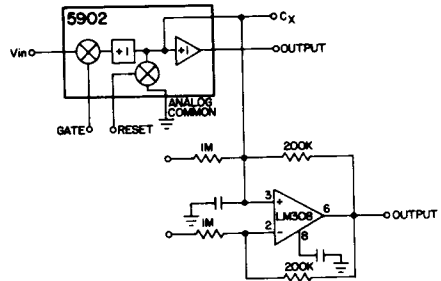
FIGURE 6: INTEGRATOR WITH PROGRAMMABLE RESET LEVEL
