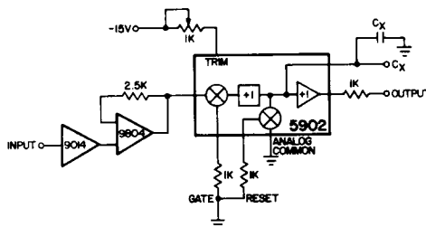
FIGURE 8: PEAK MEASUREMENT OF ABSOLUTE VALUES
