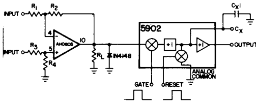
FIGURE 5: PEAK SENSE & HOLD WITH GAIN
