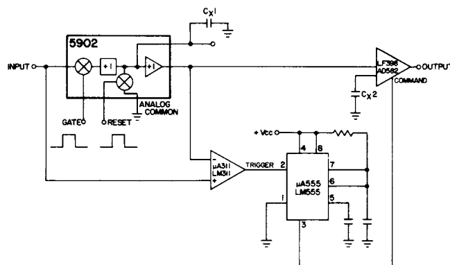
FIGURE 7: FAST ACQUISITION PEAK SENSE & HOLD WITH LOW DROOP RATE
