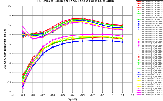
XUI009-BD_5samples: LSB Conv Gain (dB) and IIP3 (dBm) vs. Vg1 (V) IF1_ONLY = -3dBm per Tone, 2 and 2.1 GHz, LO = 2dBm
