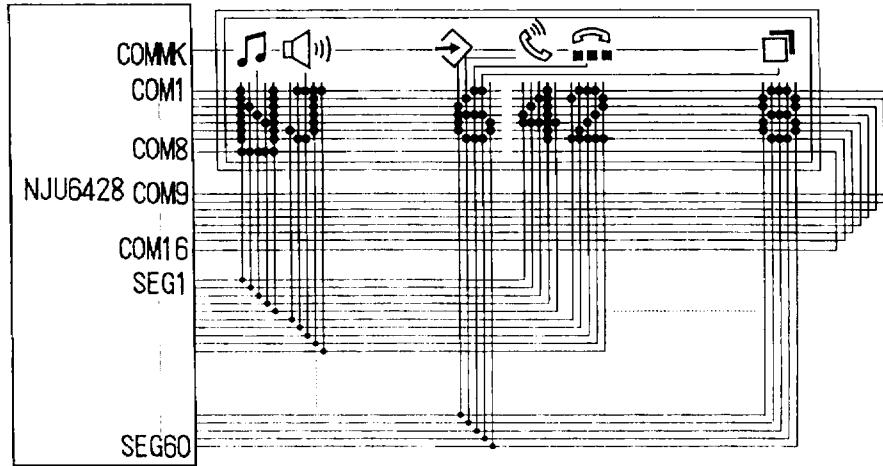
(1) 24-character 1-line WITH iCON Display Example (NJU6428)
