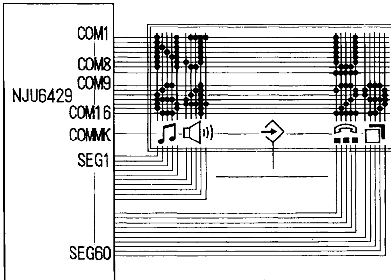
(2) 12-character 2-line with Icon Display Example (NJU6429)
