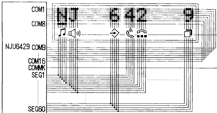
(2) 24-character 1-line WITH iCON Display Example (NJU6429)
