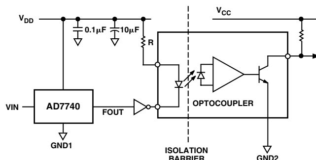
Figure 11. Opto-Isolated Application
