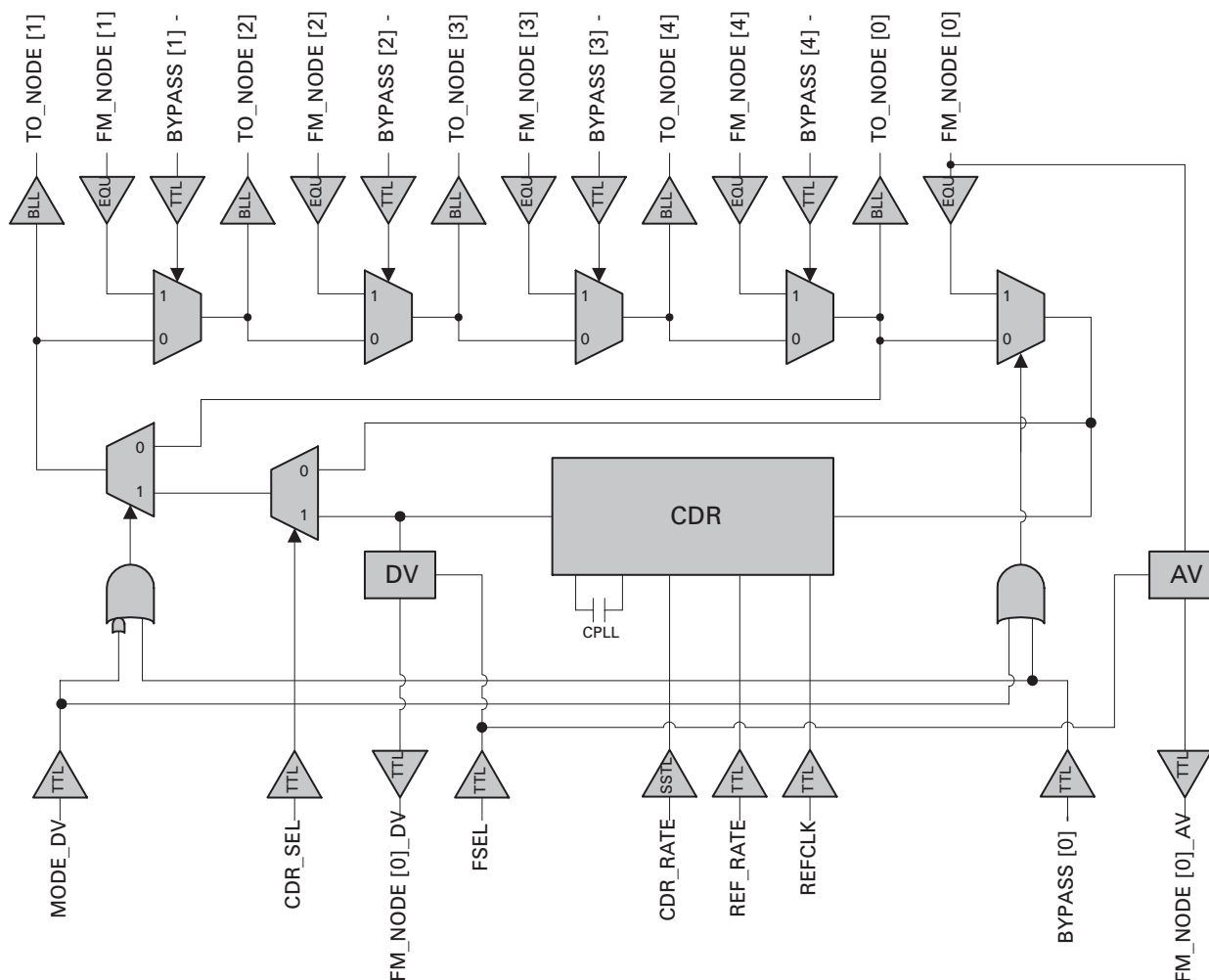
Figure 1 - Block Diagram of HDMP-0552
