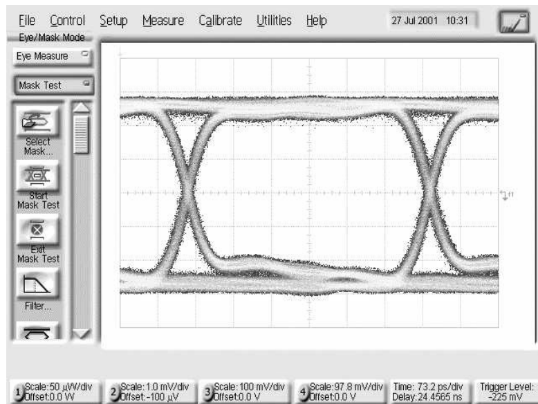
Figure 7 - Eye Diagram obtained differentially at 2.125 Gb/s FROM NODE(0) TO NODE(2) with 50 Ω termination
