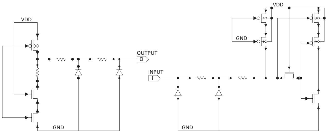
Figure 5 - Simplified Digital I/O Circuit Diagrams
