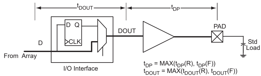
FIGURE 2-5: OUTPUT BUFFER MODEL AND DELAYS (EXAMPLE)
