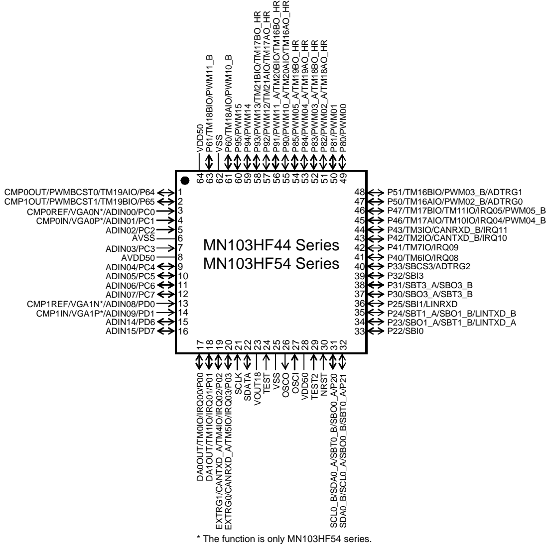
Figure:1.4.5 Pin Configuration of MN103HF44/54 Series
