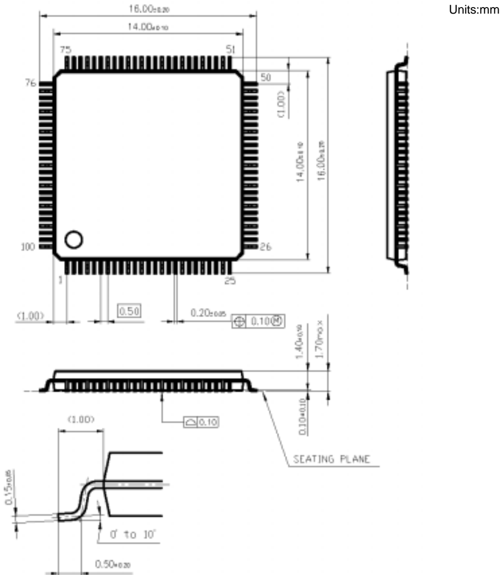
Figure:1.7.3 Package Dimension of 100 pin LQFP
