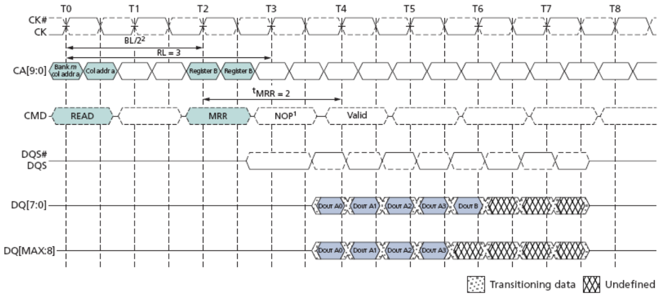
Read to MRR timing example: RL=3, t MRR=2
