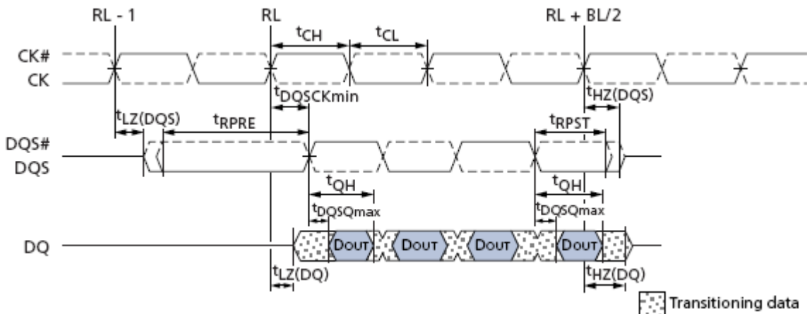
Data output (Read) timing ( t_{\text{DQSK}_{\text{min}}} ), BL=4
