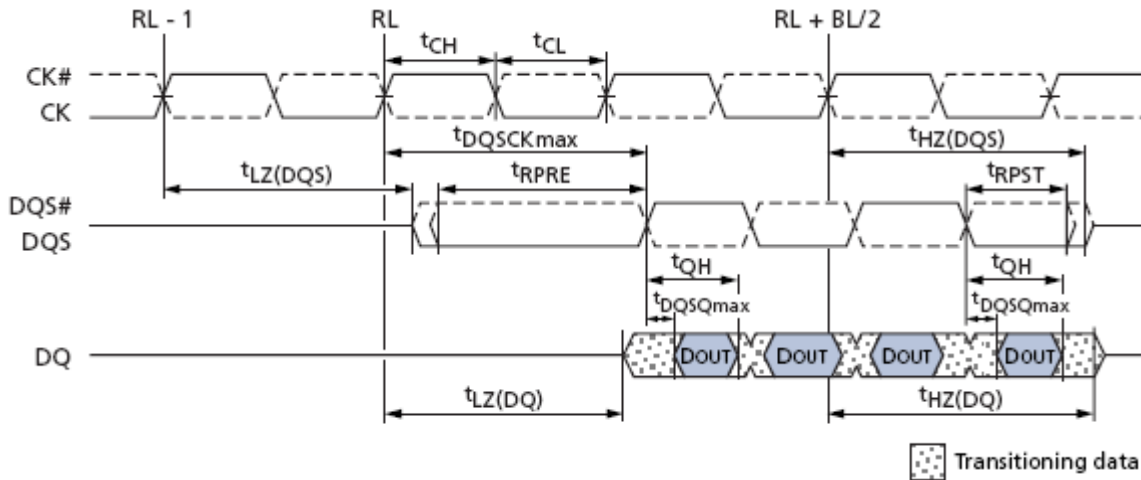
Data output (Read) timing ( t_{\text{DQSK}_{\text{max}}} )
