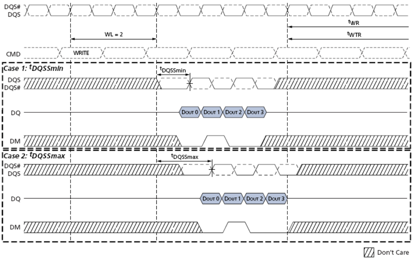
Write data mask: WL=2, BL=4, second DQ masked
