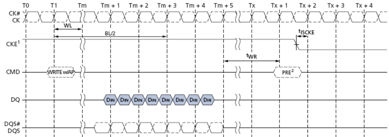
Write with Auto-precharge to Power-Down entry
