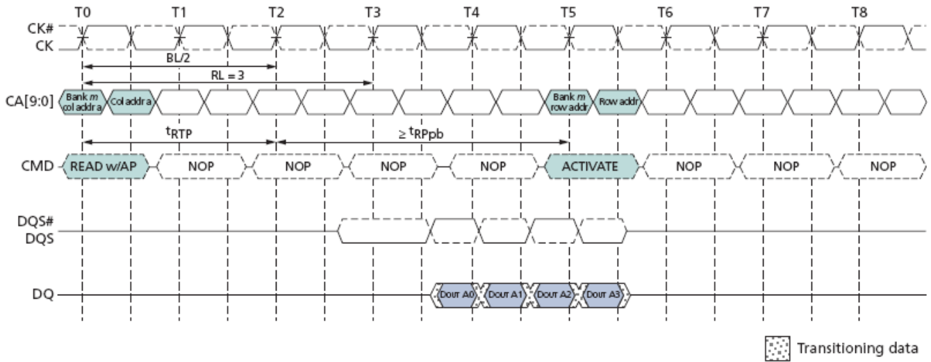
Burst Read with Auto-Precharge: RL=3, BL=4, RU(t_{RTP}(\min)/CK)=2
