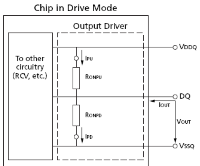
Output Driver
