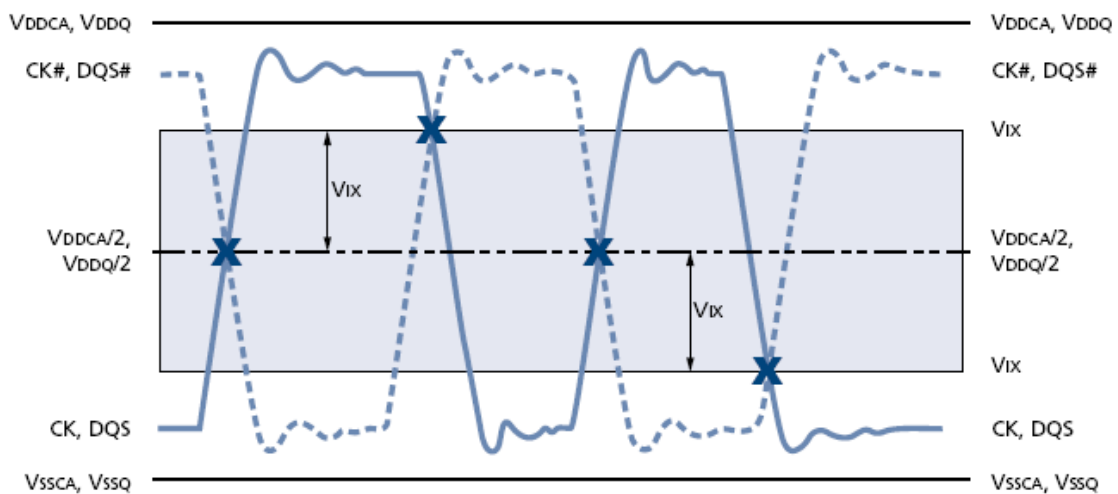
V_{IX} definition
