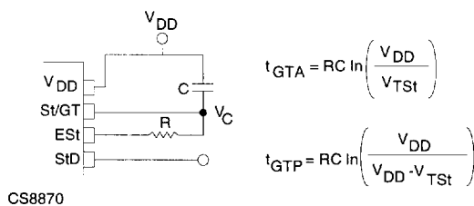
Figure 2 - Basic Steering Circuit
