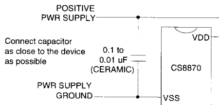
Figure 7. Power Supply Decoupling
