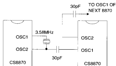
Figure 6 - Oscillator Interconnection
