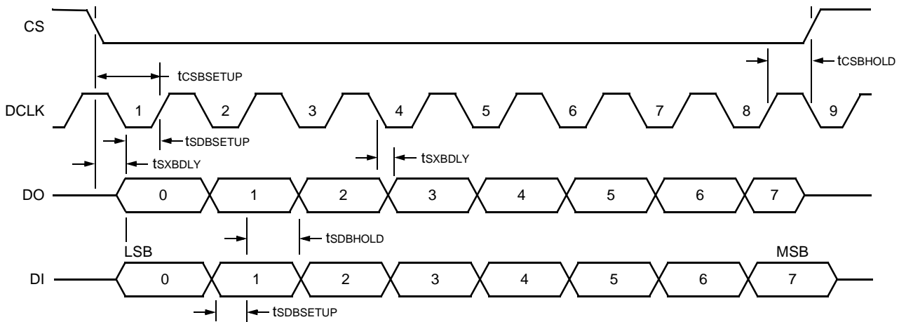
Figure 22. Byte-by-Byte Mode Timing
