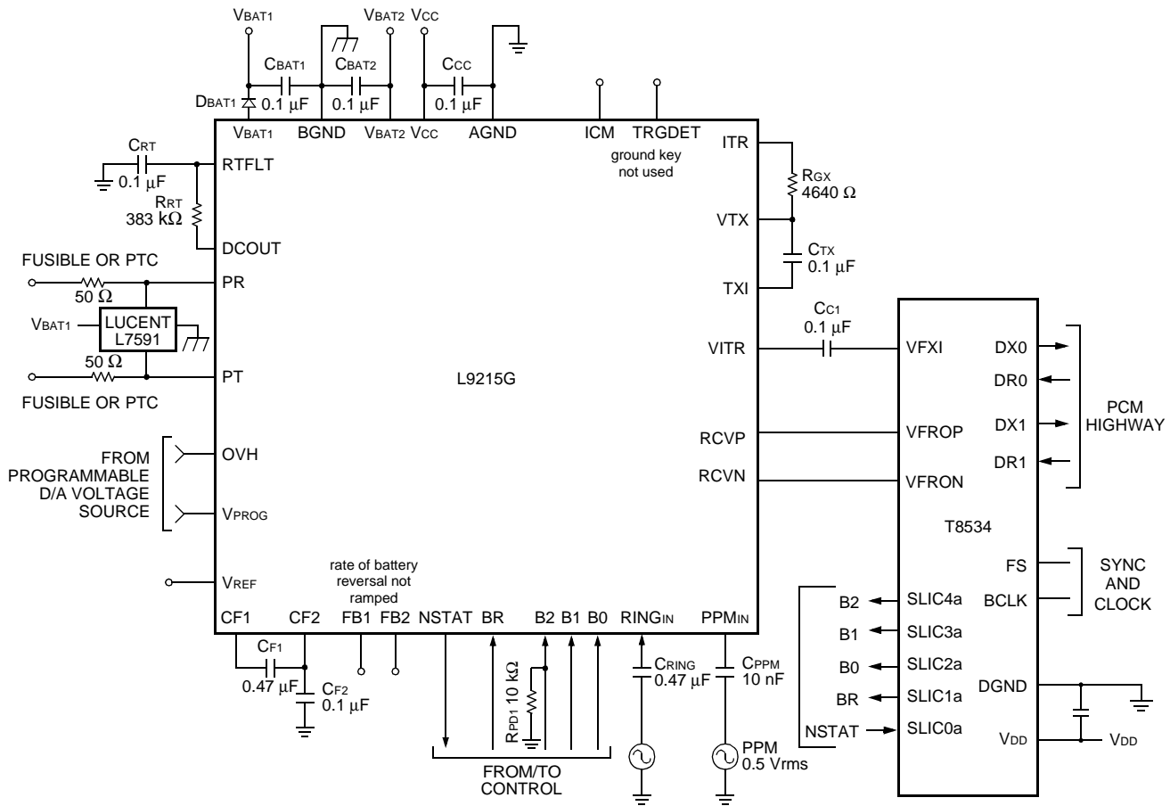
Figure 24. POTS Interface
