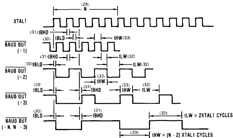
BAUDOUT TIMING
