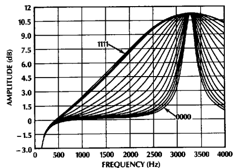
Figure 5. Typical Bandwidth Filter Response — NL/L = 0
