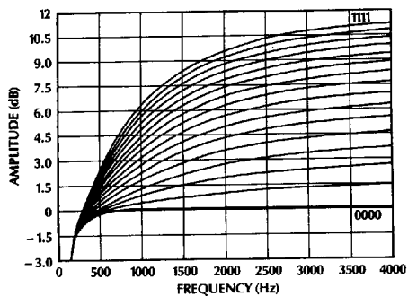
Figure 3. Typical Slope Filter Response — NL/L = 1
