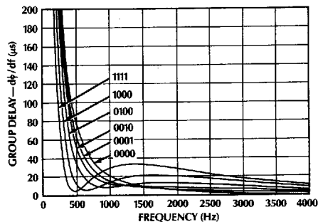
Figure 3. Typical Slope Filter Response — NL/L = 1
