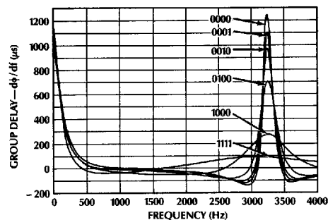
Figure 5. Typical Bandwidth Filter Response — NL/L = 0
