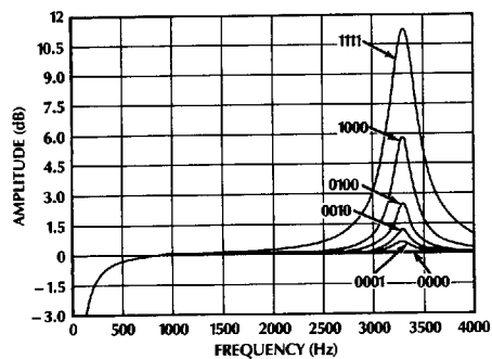
Figure 4. Typical Height Filter Response — NL/L = 0
