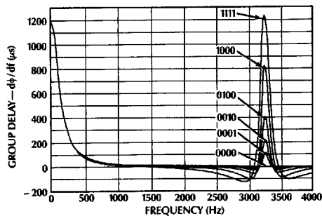
Figure 4. Typical Height Filter Response — NL/L = 0
