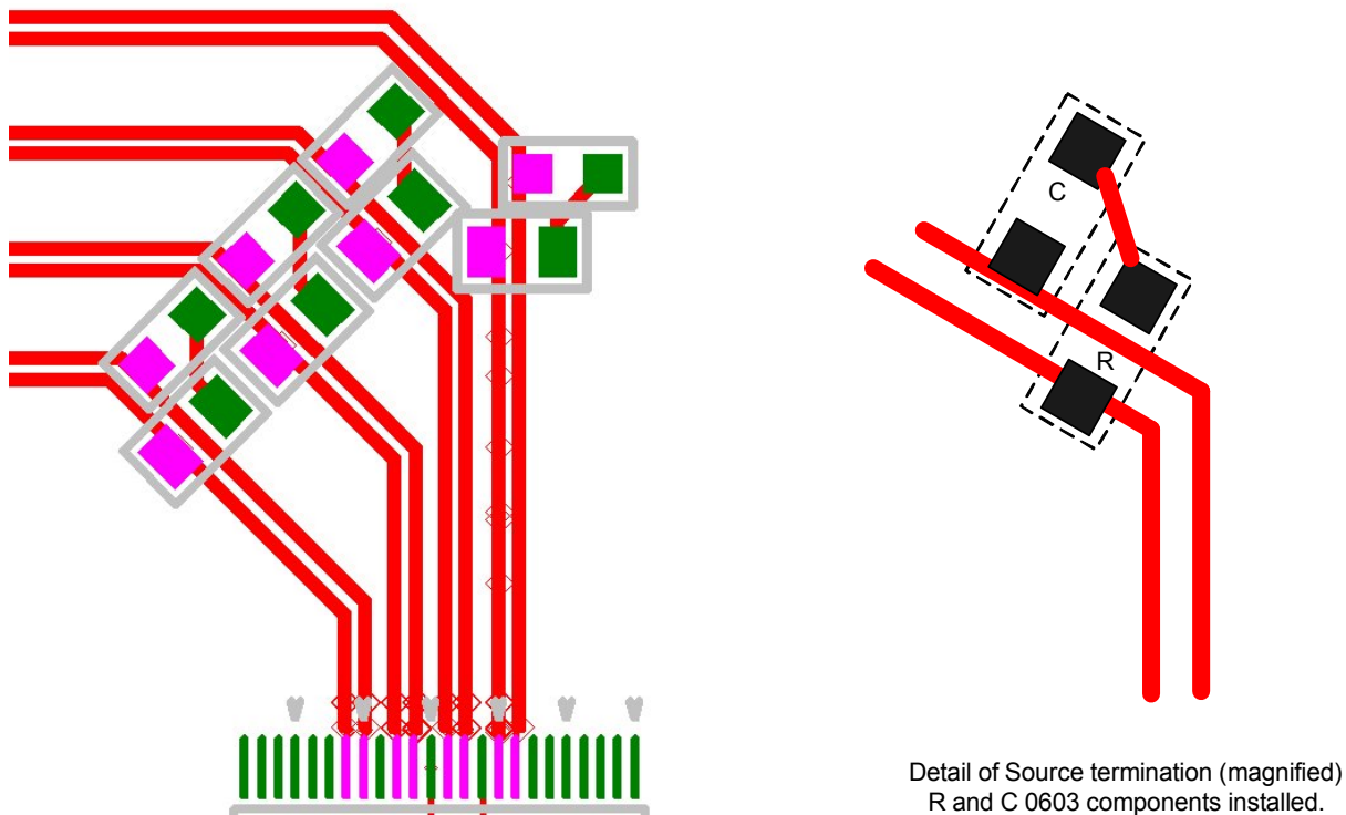
Figure 23. Source Termination Layout Illustration
