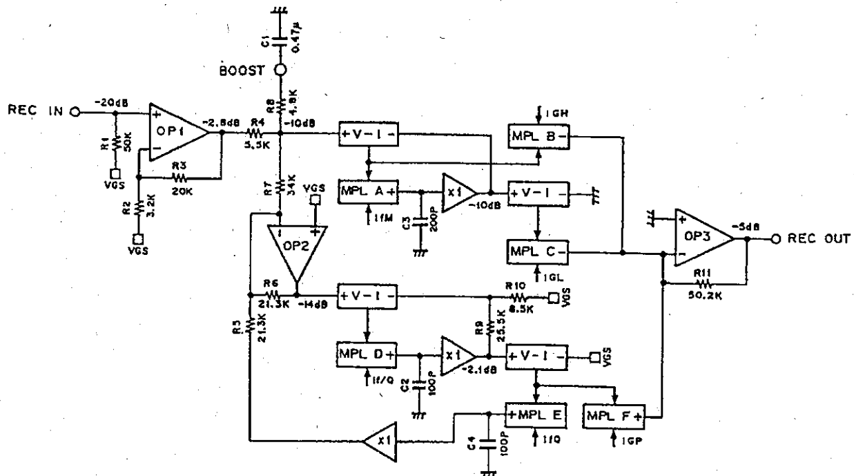
Fig. 1. CX1579 functional circuit block diagram
