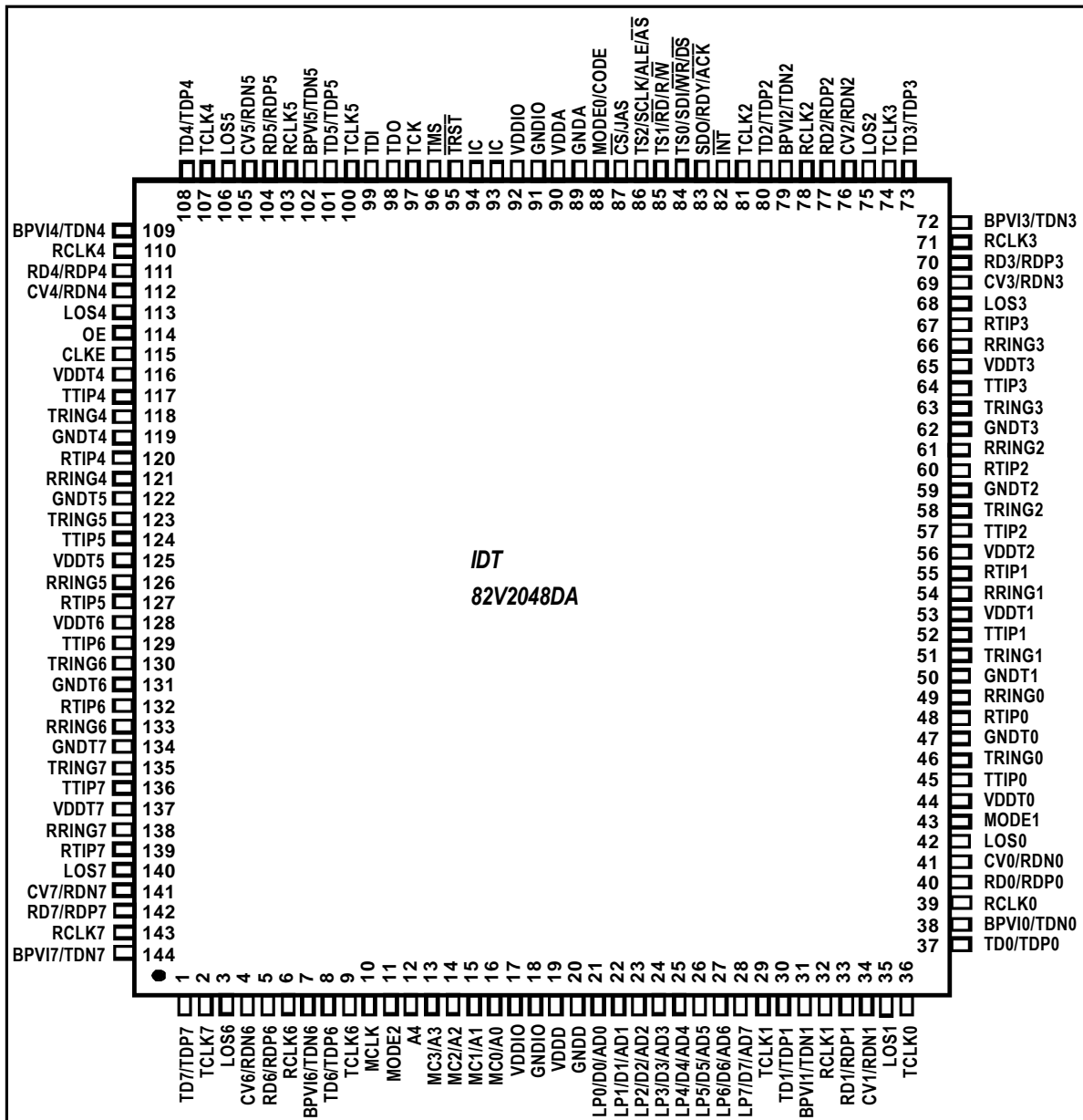
Figure - 2a. PQFP144 Package Pin Assignment
