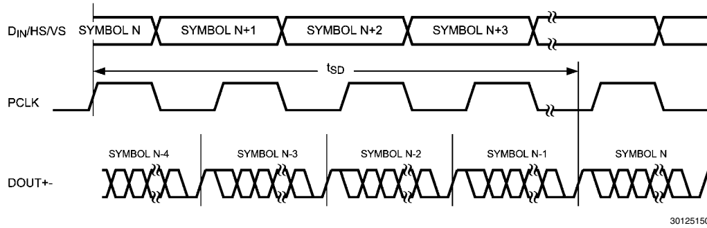
FIGURE 11. Serializer Delay
