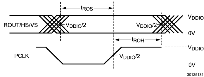
FIGURE 15. Deserializer Output Setup/Hold Times
