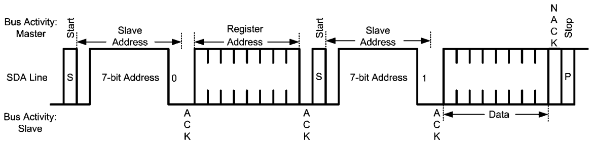
FIGURE 21. Read Byte
