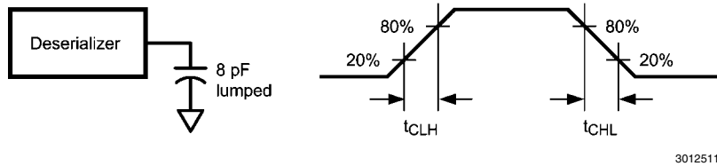
FIGURE 13. Deserializer LVCMOS Output Load and Transition Times
