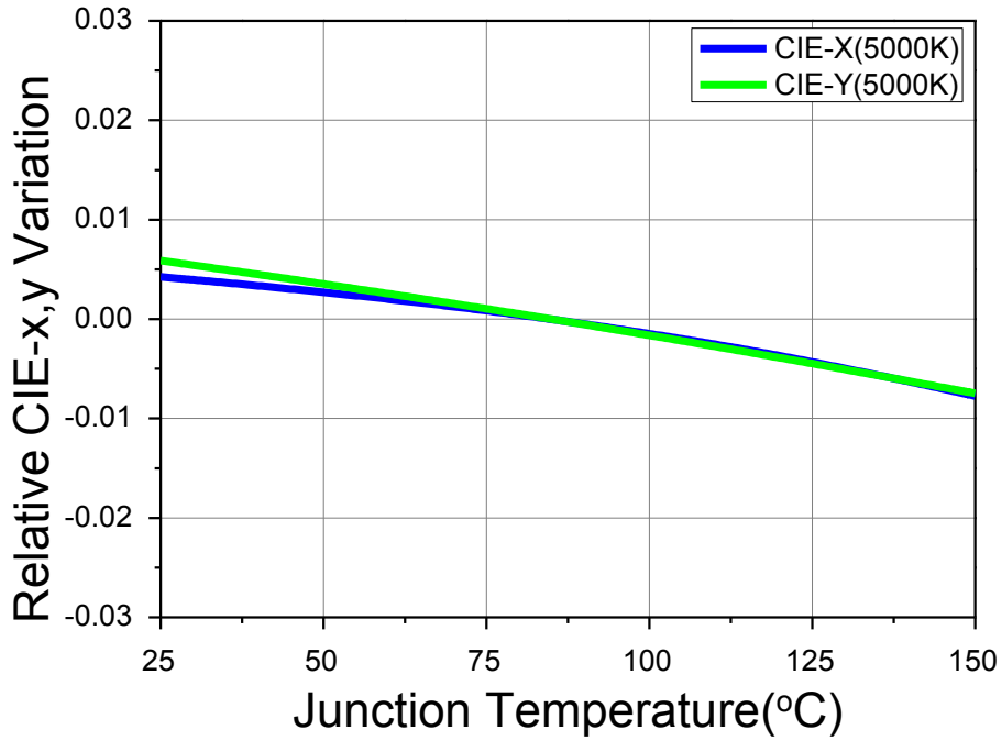
Fig 7. Junction Temperature vs. CIE x,y Shift, I_f=0.9A (CRI70, 5000K)
