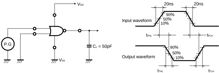
Fig.2 Switching characteristics measurement circuit
