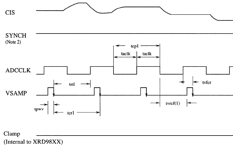
Graph 8. 1 Channel S/H Mode – No Clamp (DC Coupled)
