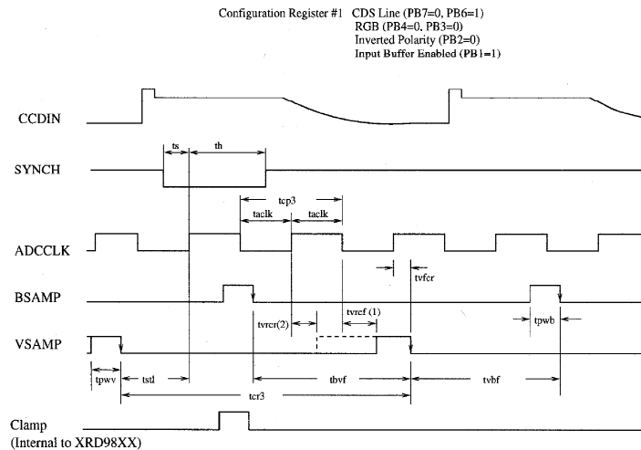
Graph 2. 3 Channel CDS Mode – Line Clamp
