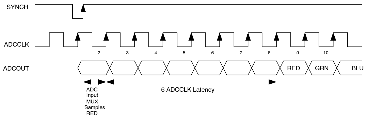
Graph 14. XRD9812 Timing For SYNCH/ADCCLK/ADCOUT
