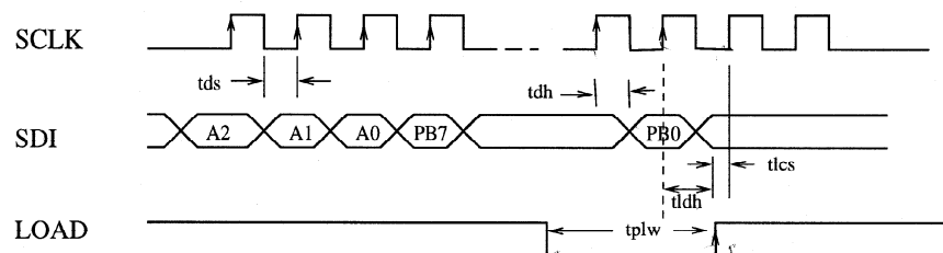
Graph 9. Write Timing
