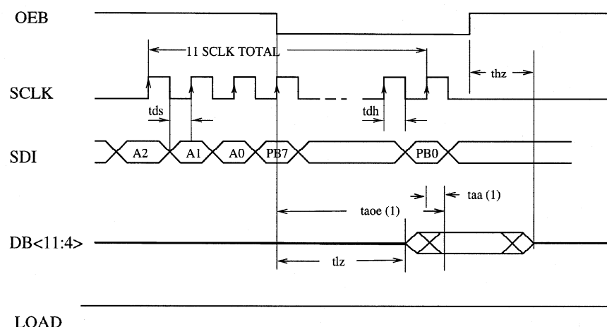
Graph 10. Read-Back Mode Timing
