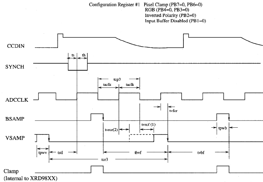
Graph 1. 3 Channel CDS Mode – Pixel Clamp
