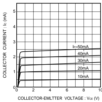
Fig.10 Output characteristics
