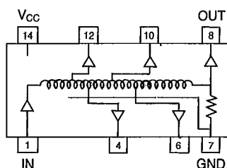
P Internal wiring
