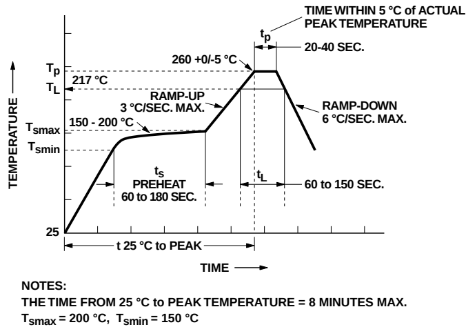
Figure 2. Pb-Free IR Profile.
