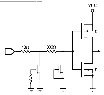
FIGURE 3. OUTPUT CIRCUIT
