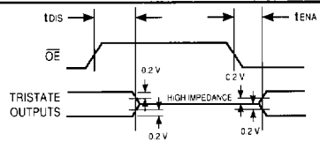
FIGURE 4. THRESHOLD LEVELS
