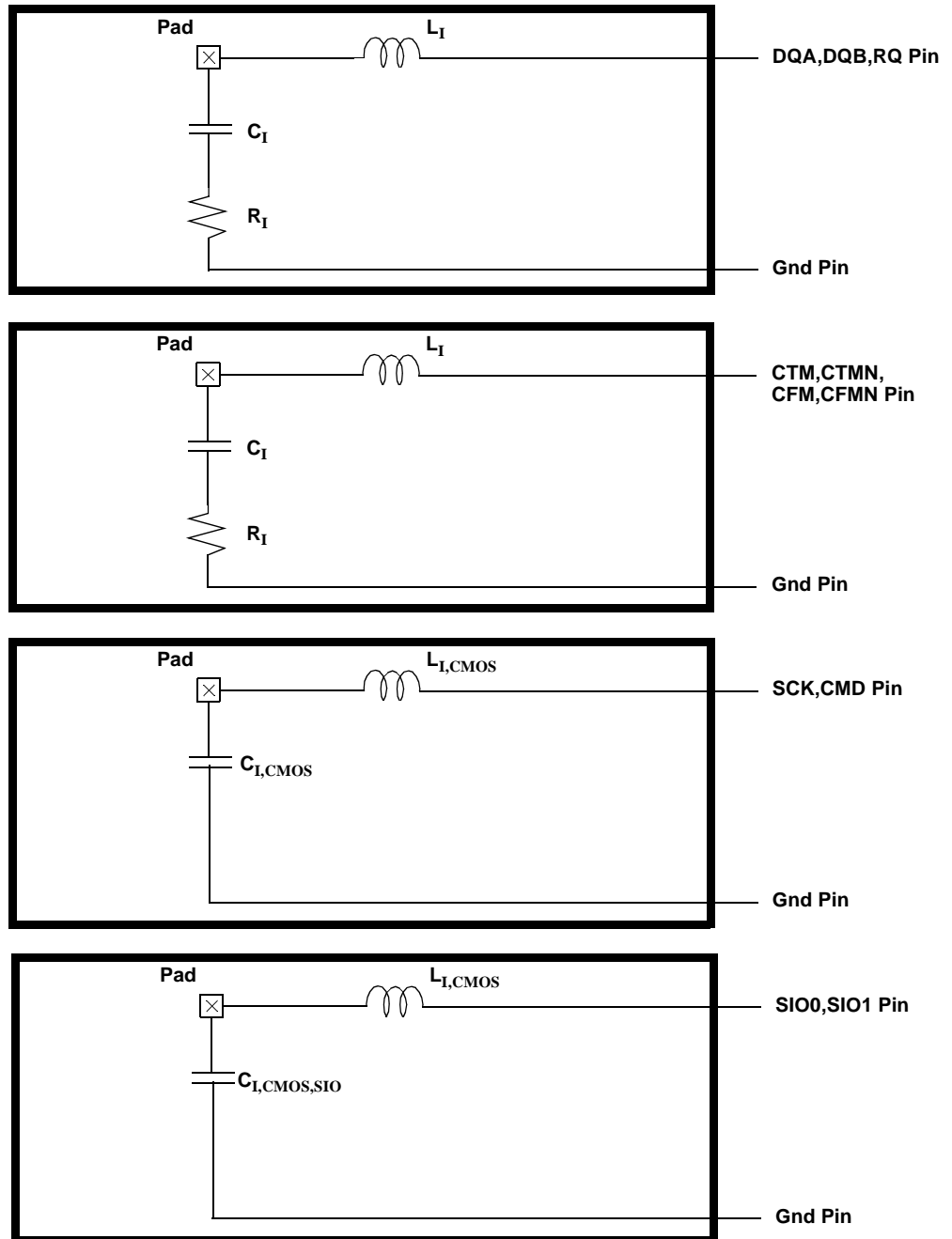
Figure 1: Equivalent Load Circuit for RSL Pins
