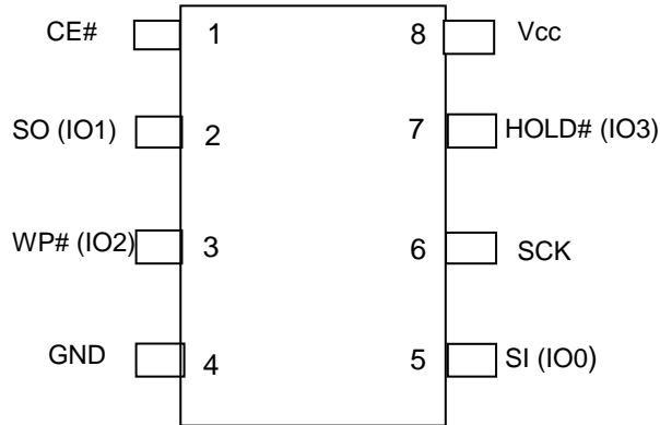
8-Pin SOIC/VVSOP
