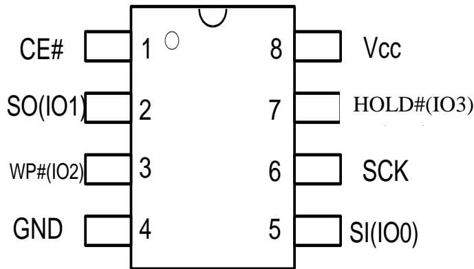
8-Pin PDIP
