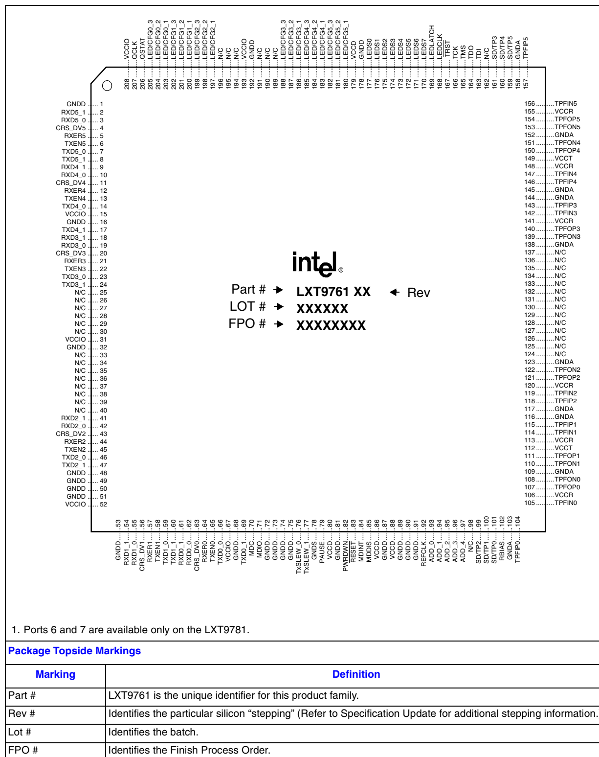
Figure 4. LXT9761 PQFP Pin Assignments
