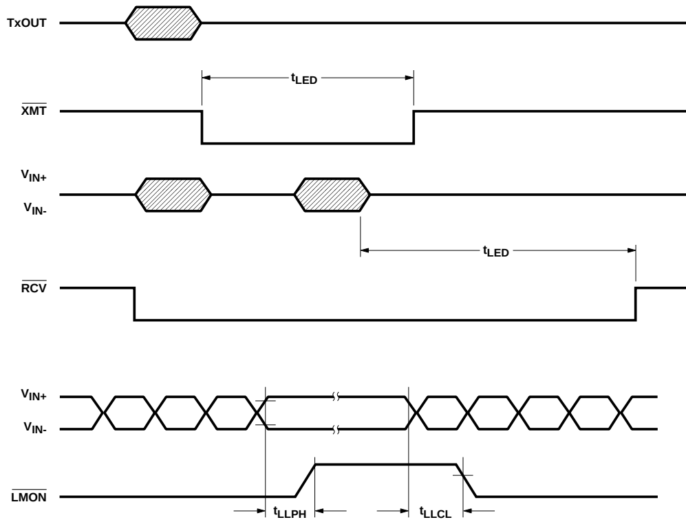
Figure 13. LED Timing.
