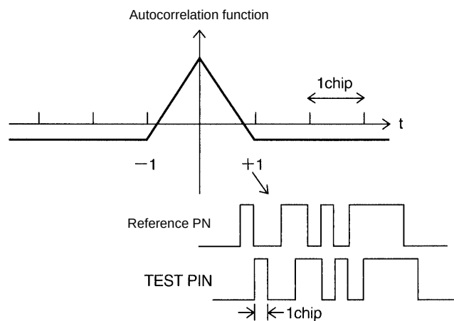
Fig. 4 Autocorrelation function
