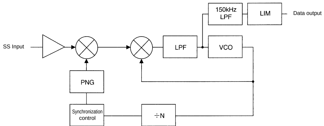
Fig. 3 The reception block
