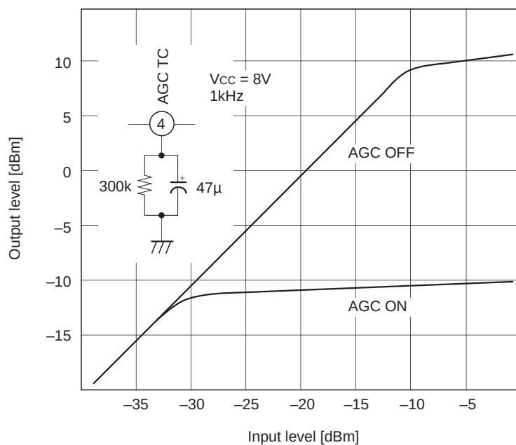
AGC output characteristics
