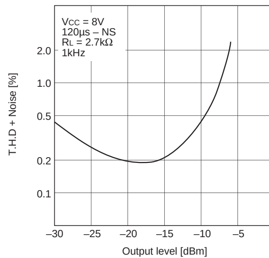
Playback equalizer total harmonic distortion
