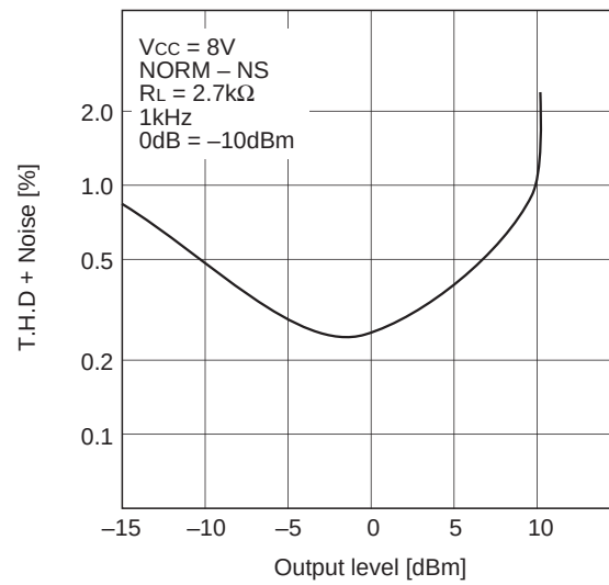
Recording equalizer total harmonic distortion
