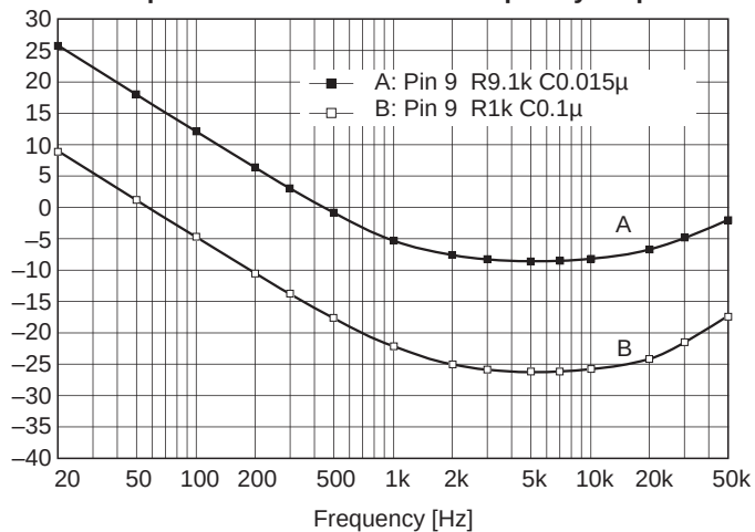
AMS quiescent detection level frequency response
