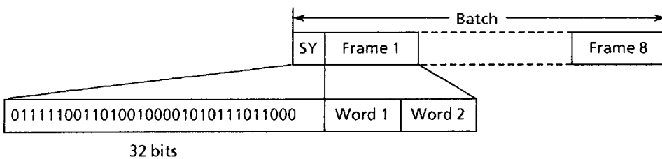
Figure 7 Batch configuration
