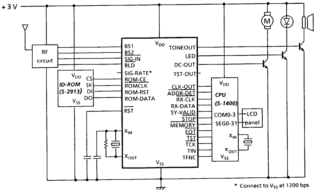
Figure 34 Application circuit example: Display pager
