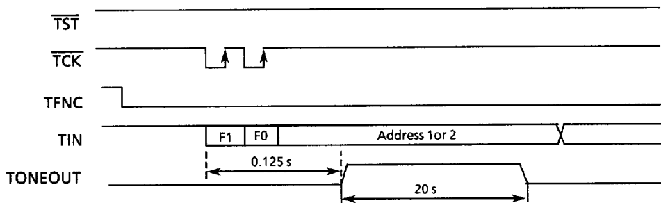
Figure 29 Call forcible output timing
