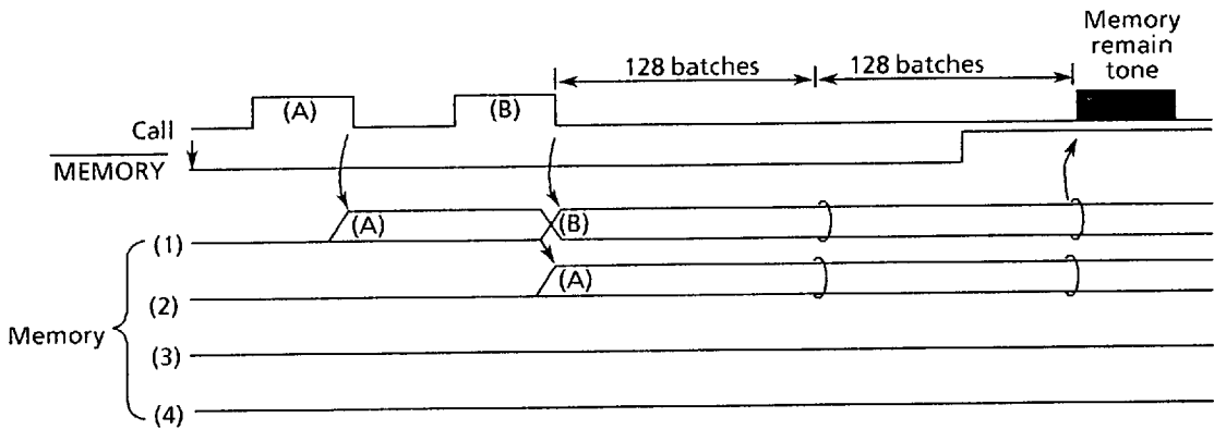
Figure 25 Memory remain tone timing
