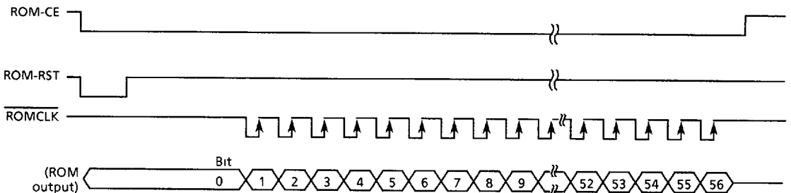
Figure 31 Mask option (S-2100 mode) ID-ROM interface
