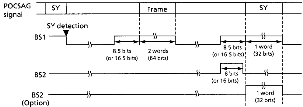
Figure 19-2 Battery saving
