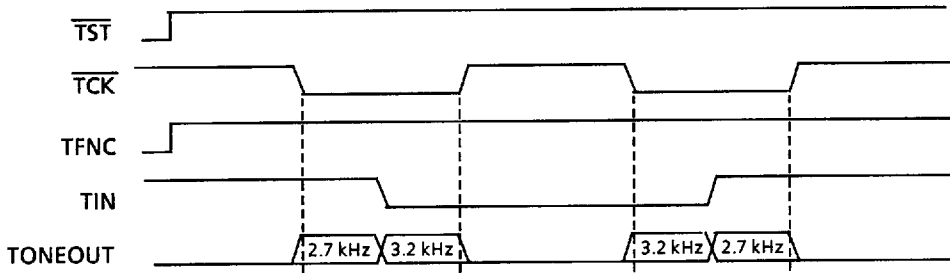
Figure 28 Tone forcible output timing
