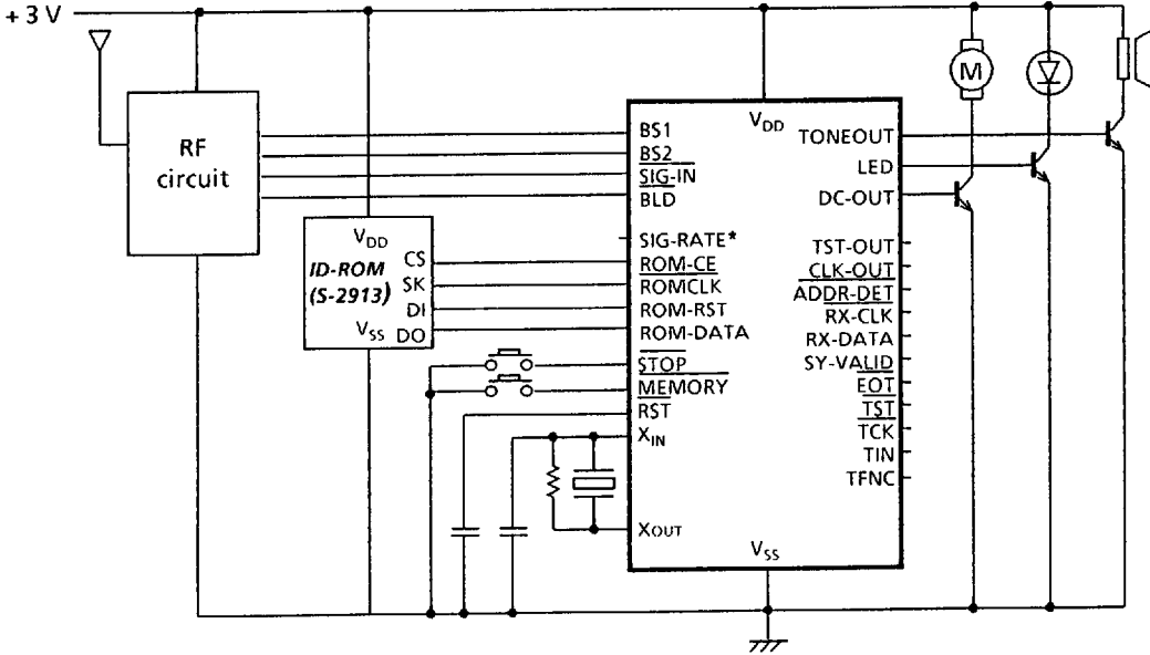
Figure 33 Application circuit example: Tone-only pager
