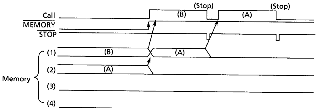
Figure 24 Scroll timing
