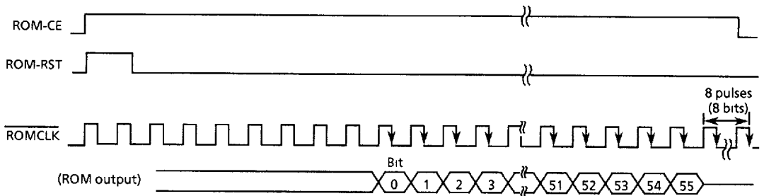
Figure 30 Standard (S-2913 compatible mode) ID-ROM interface
