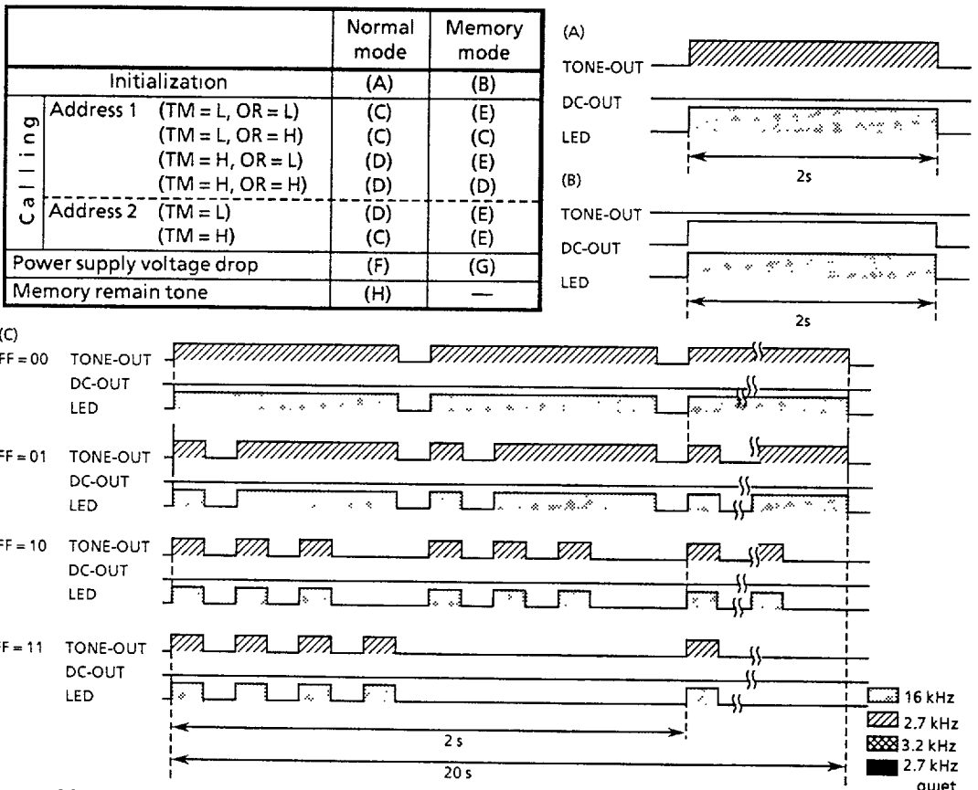
Figure 18-1 Relationship between output waveforms of TONE-OUT, LED and DC-OUT
