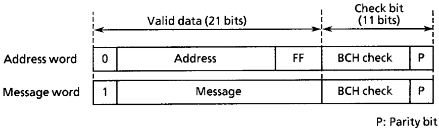
Figure 21 Address and message word configuration
