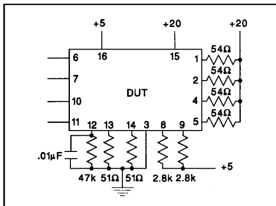
Figure 3. Test Circuit
