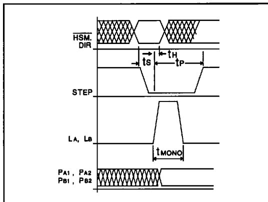
Figure 4. Timing Waveforms
