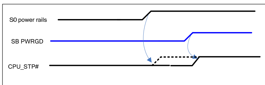
Figure 4-10: CPU_STP# De-asserted when SB PWRGD Asserted
