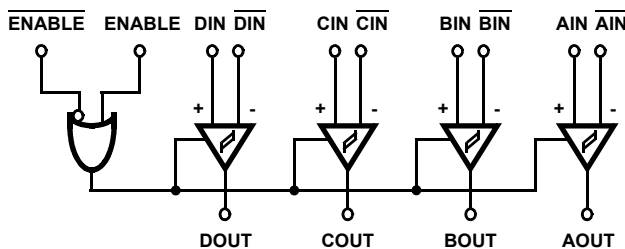
FIGURE 1. LOGIC DIAGRAM
