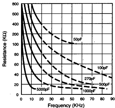
Resistance vs Oscillator Frequency - ED9R, ED15R
