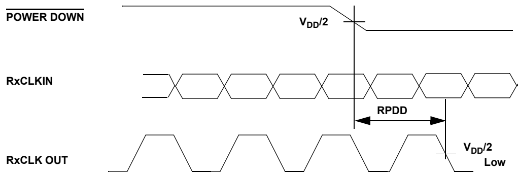
Figure 8. UT54LVDS218 Phase Lock Loop Set Time
