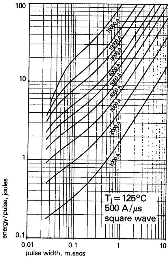
Figure 5 Energy/pulse v. pulse width
