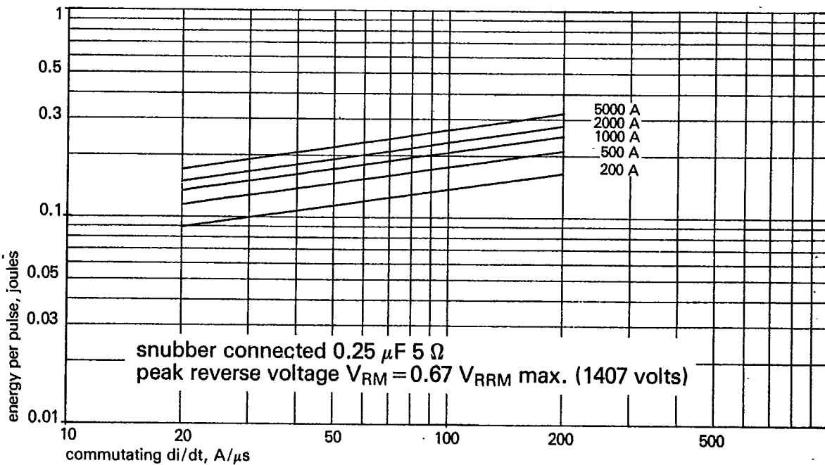
Figure 7 Max. reverse recovery energy loss per pulse at 125^\circ\text{C} junction temperature and V_{RM} = 1407 \text{ volts}
