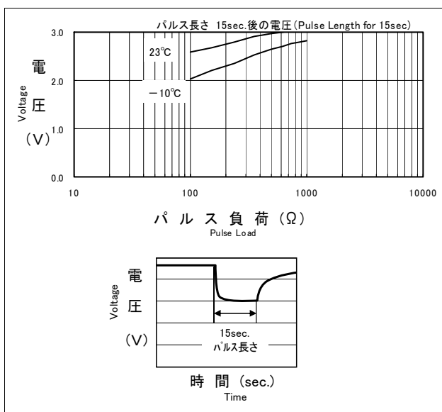
Discharge Characteristics on Pulse Load (Discharge depth 40%)
