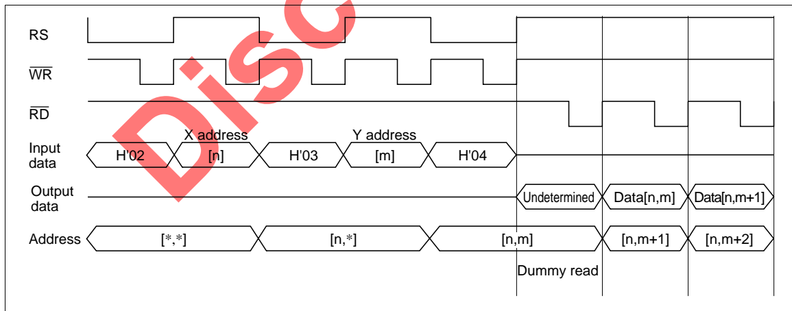
Figure 10 Display RAM Read Sequence
