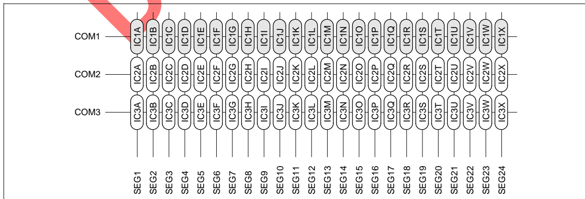
Figure 21 Annunciator Display Data and Display Positions
