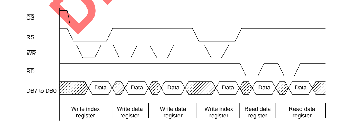
Figure 3 8-Bit Data Transfer Sequence
