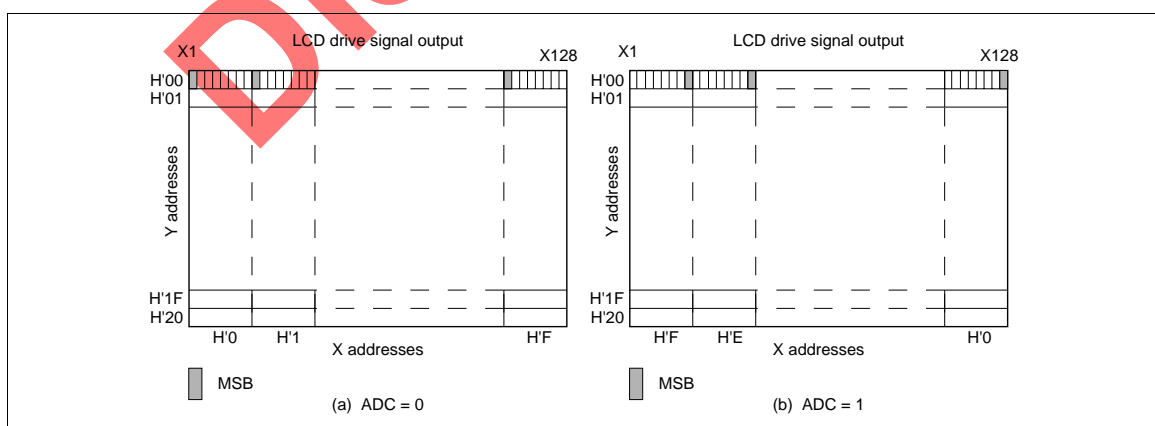
Figure 9 Display RAM Configuration
