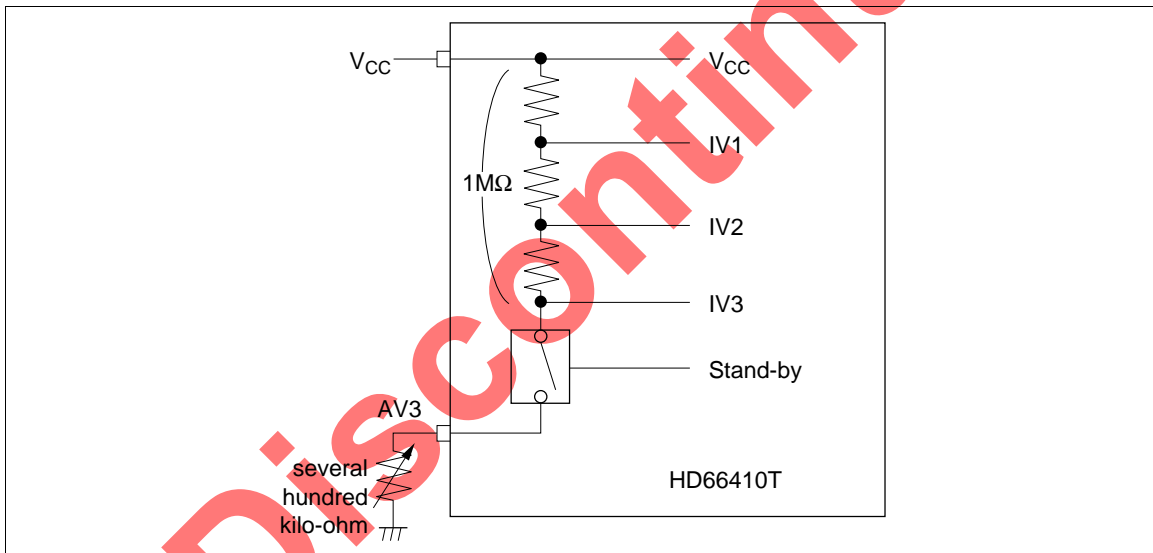
Figure 24 Power Circuit for Annunciator
