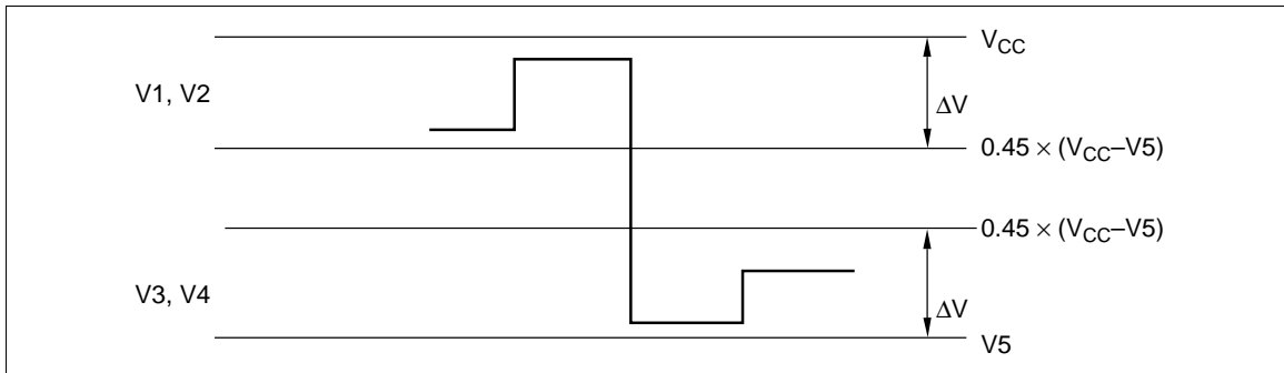
Figure 38 Limitation of V1 to V4 Levels
